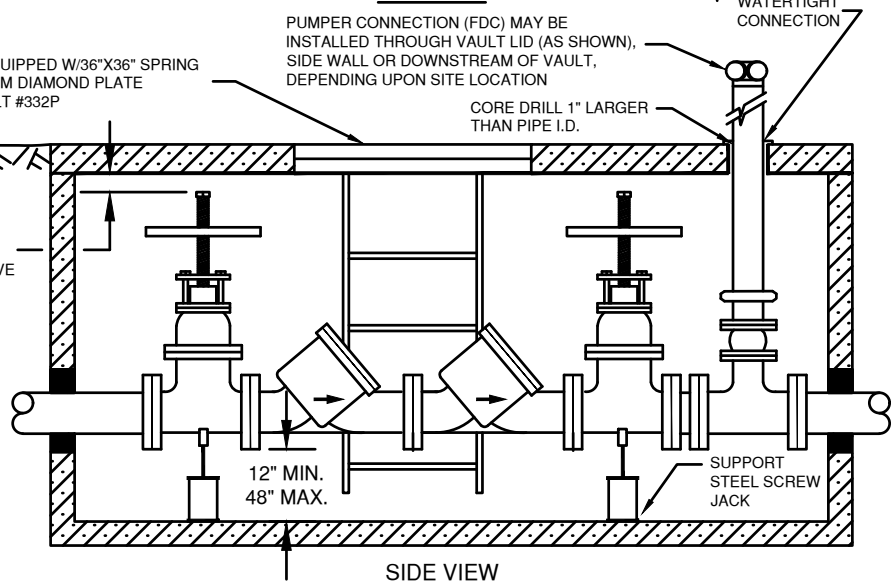
SIDE VIEW
