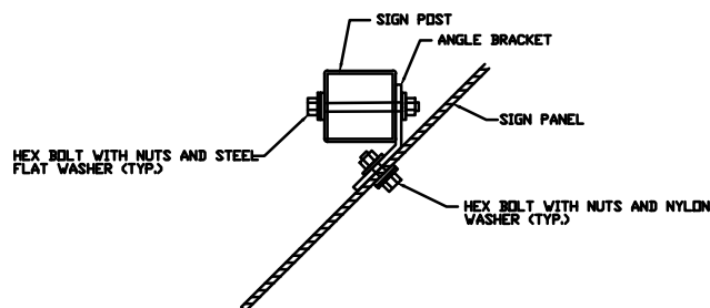
DETAIL 1
