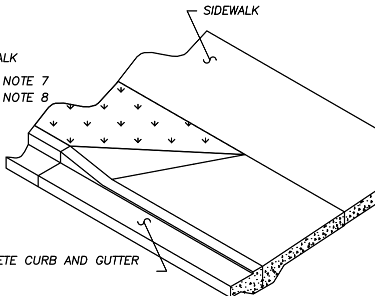
APPROACH TYPE I - HALF ISOMETRIC
