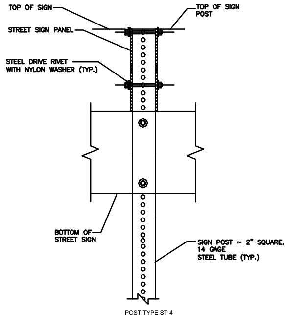
STREET NAME SIGN INSTALLATION DETAIL
